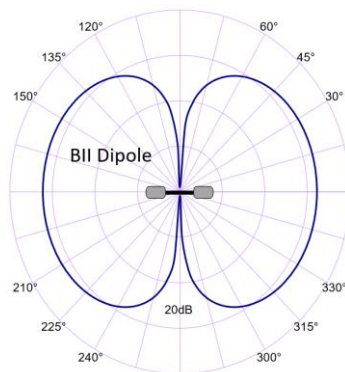
"Figure 8" Pattern of a Dipole (Pressure-Gradient).
