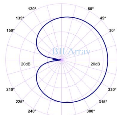
Cardioid Pattern= Omnidirectional + Dipole.
